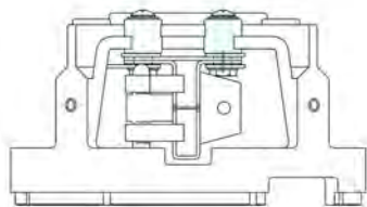
Standard anti-drive end endbell blocks critical cooling air
